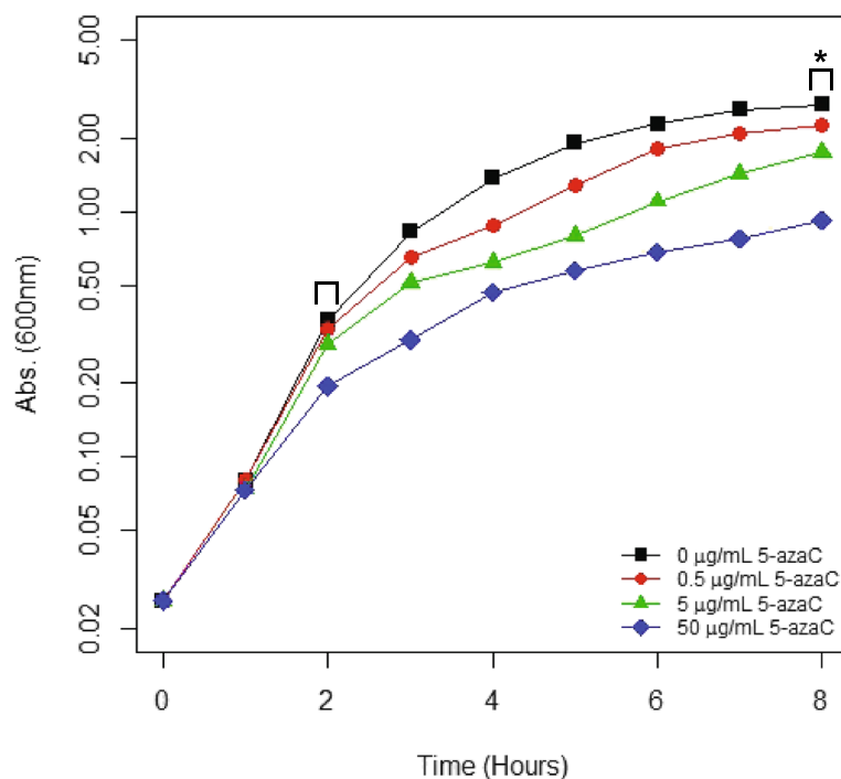
Fig. 2 The effect of 5-azaC on Escherichia coli growth in liquid media. E. coli wild-type strain BW25113 was grown in LB at 37 °C in the absence of 5-azaC (black squares), the presence of 0.5 \mu\text{g}/\text{mL} 5-azaC (red circles), 5 \mu\text{g}/\text{mL} 5-azaC (green triangles) and 50 \mu\text{g}/\text{mL} 5-azaC (blue diamonds) for eight hours. At every hour, each culture was analyzed by spectrophotometry at 600 nm. The data are from three biological replicates ( n = 3 ). Error bars representing standard deviation are not shown to maintain clarity of the four lines. Brackets indicate time points of RNA isolation for microarray analysis, and data analyzed by ANOVA. The asterisk indicates a p -value of <0.05
